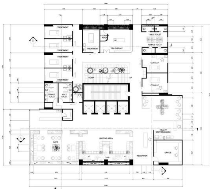
1ST FLOOR
