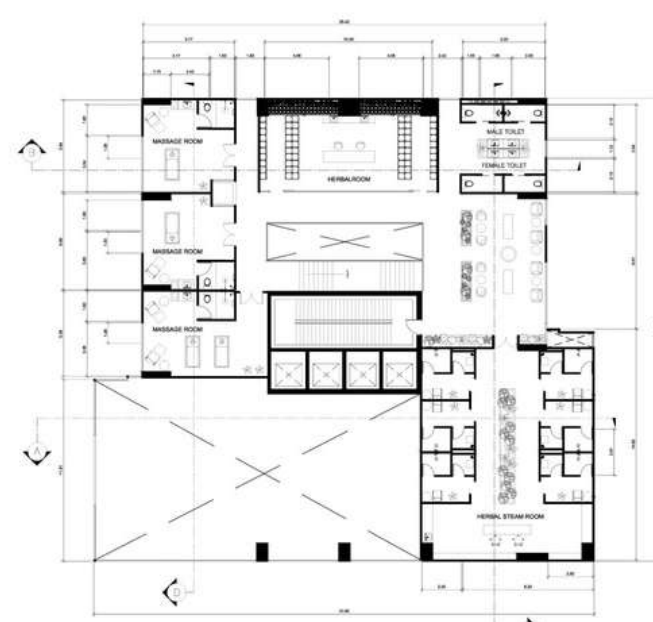
2ND FLOOR
