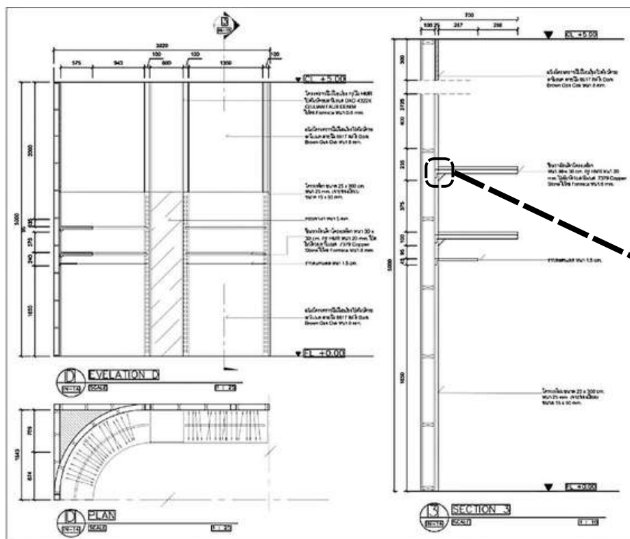
FURNITURE DESIGN PLAN
